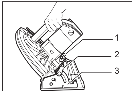
► 1. Clamp screw 2. Lever 3. Bevel scale plate
