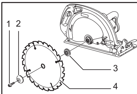
► 1. Hex bolt 2. Outer flange 3. Inner flange 4. Saw blade
